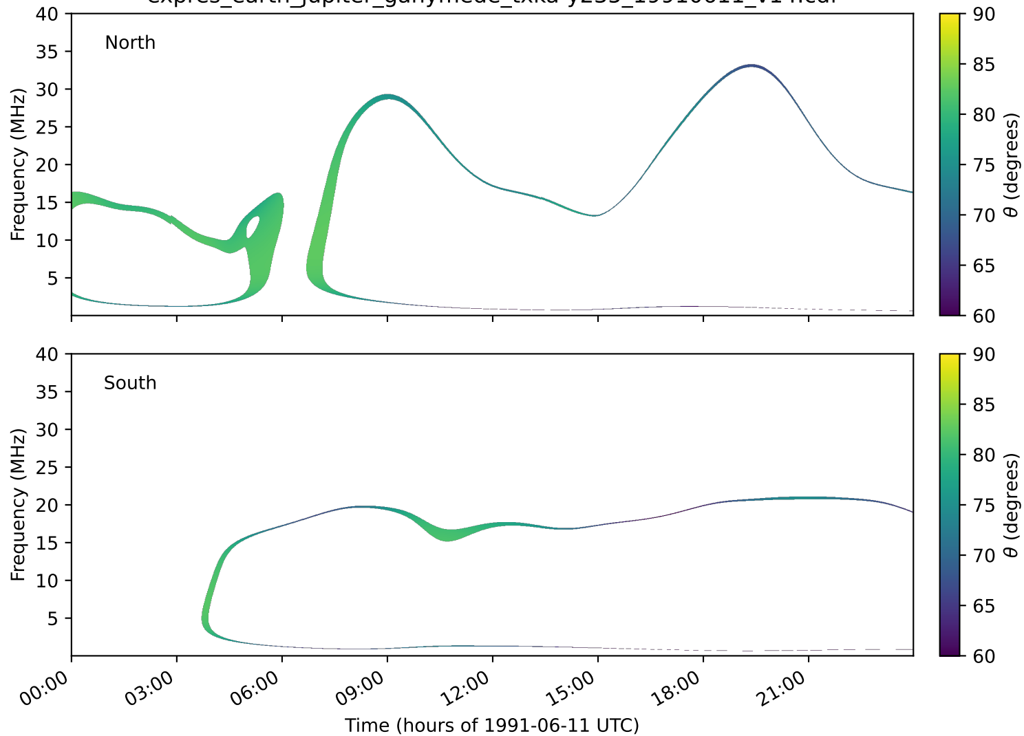
expres_earth_jupiter_ganymede_txka-y235_19910611_v14.cdf
