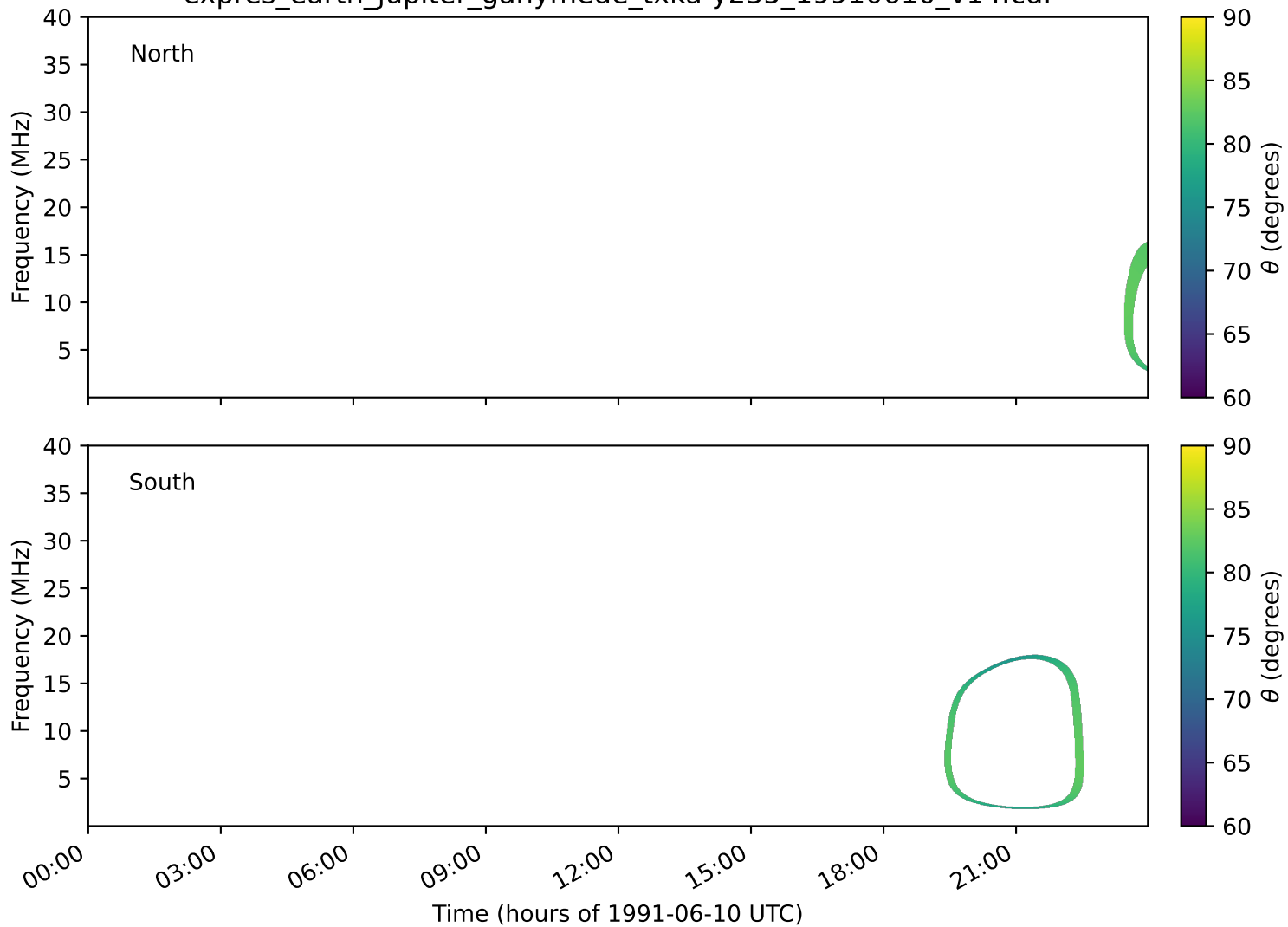
expres_earth_jupiter_ganymede_txka-y235_19910610_v14.cdf
