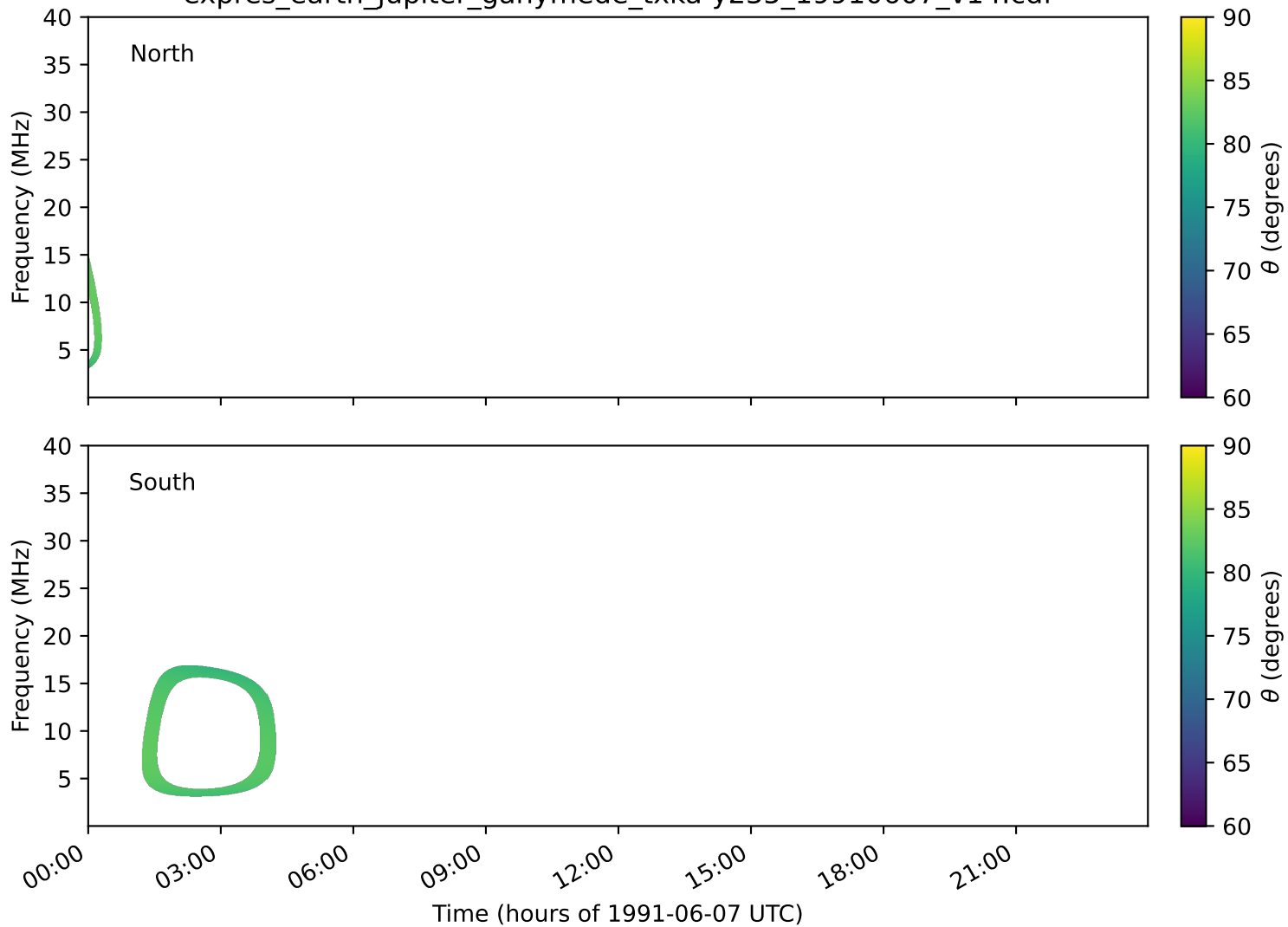
expres_earth_jupiter_ganymede_txka-y235_19910607_v14.cdf
