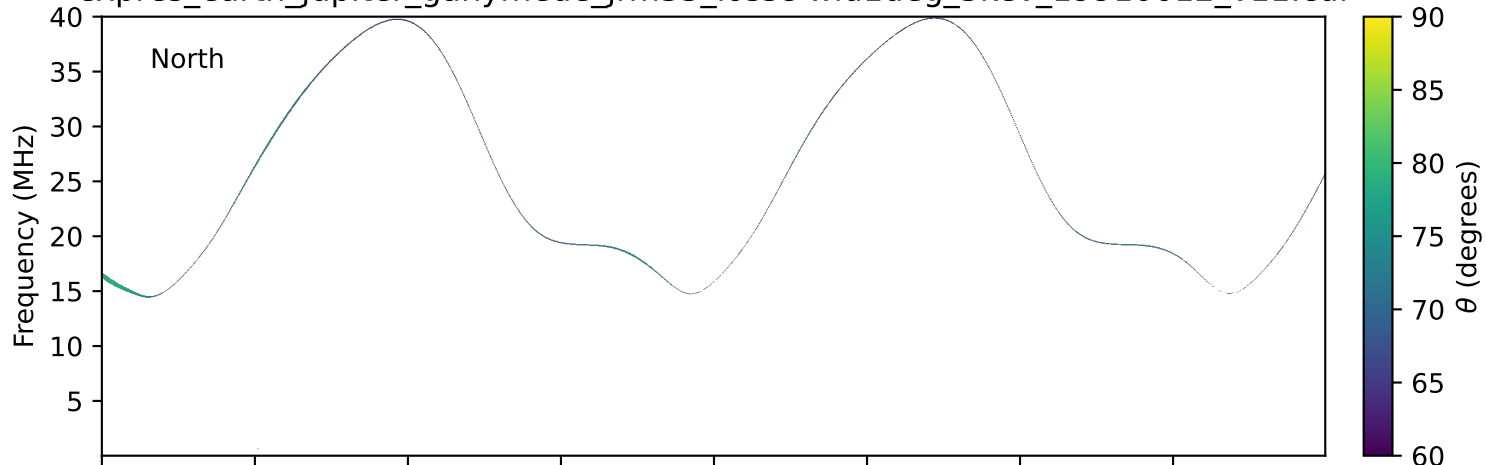
expres_earth_jupiter_ganymede_jrm33_lossc-wid1deg_3kev_19910612_v11.cdf
