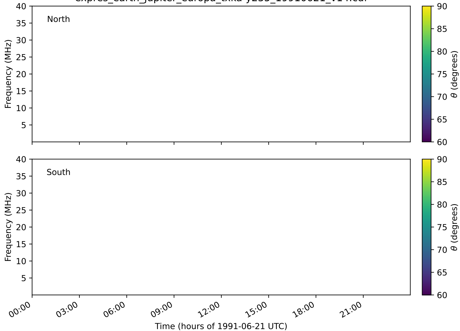
expres_earth_jupiter_europa_txka-y235_19910621_v14.cdf
