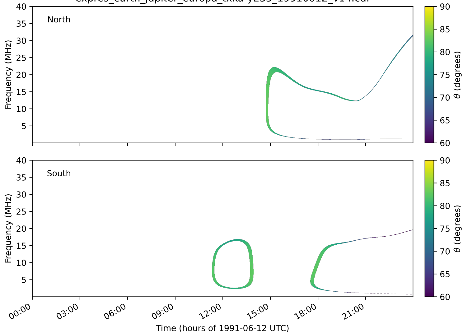
expres_earth_jupiter_europa_txka-y235_19910612_v14.cdf
