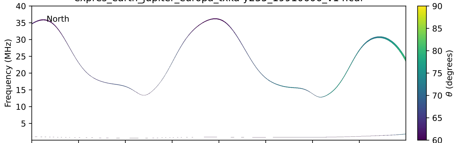
expres_earth_jupiter_europa_txka-y235_19910606_v14.cdf
