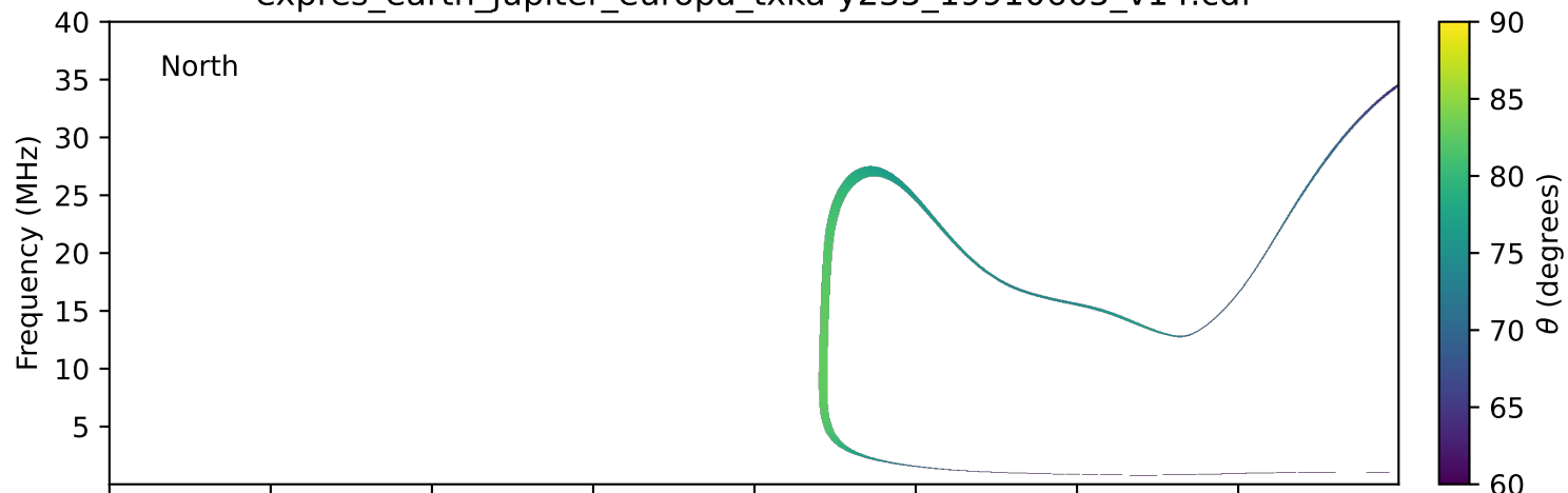
expres_earth_jupiter_europa_txka-y235_19910605_v14.cdf
