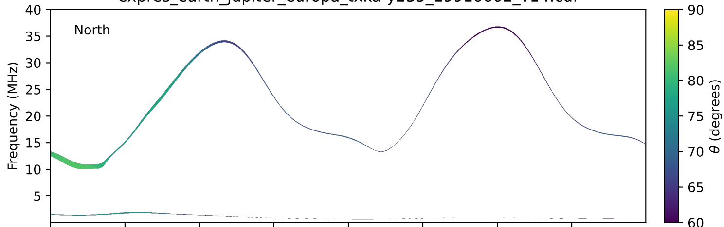
expres_earth_jupiter_europa_txka-y235_19910602_v14.cdf
