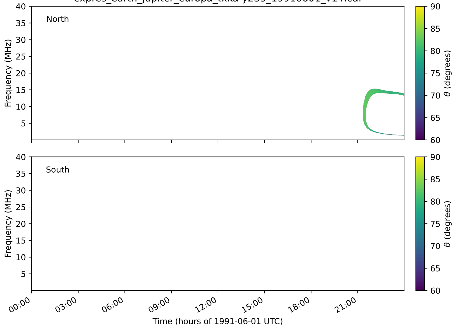
expres_earth_jupiter_europa_txka-y235_19910601_v14.cdf
