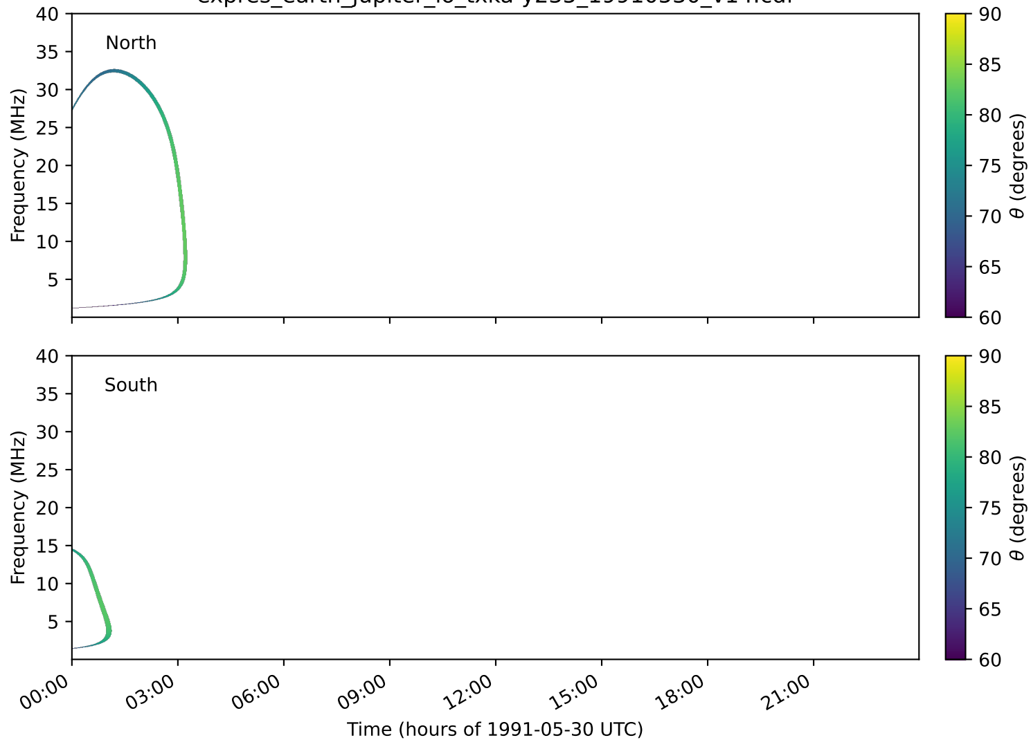
expres_earth_jupiter_io_txka-y235_19910530_v14.cdf
