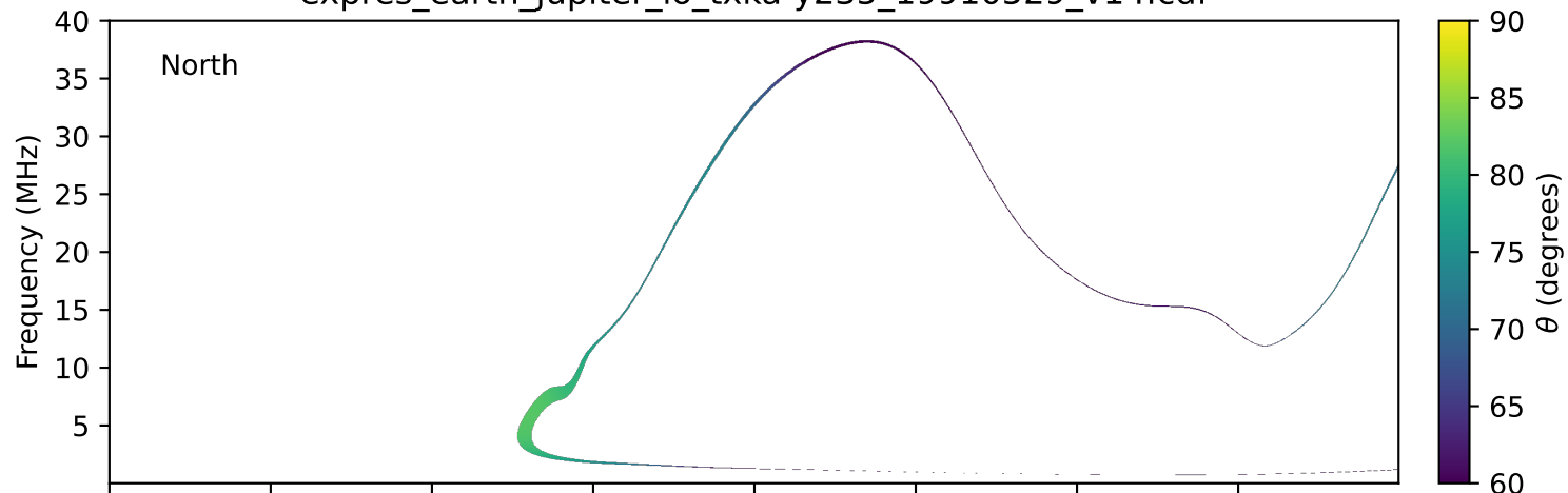
expres_earth_jupiter_io_txka-y235_19910529_v14.cdf
