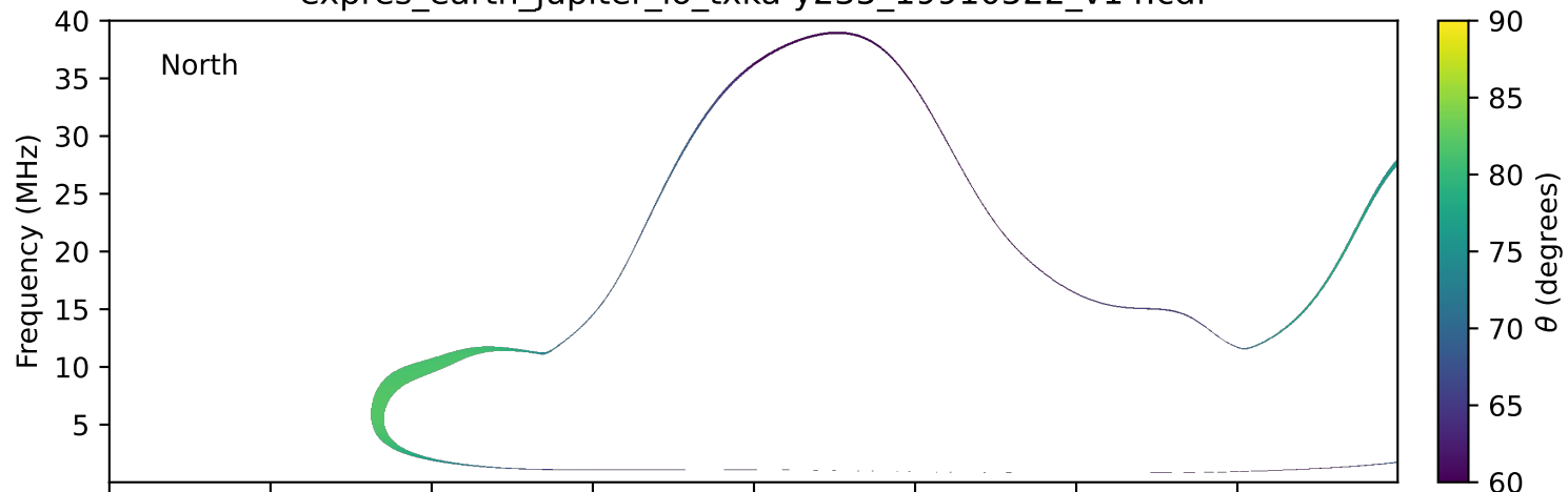
expres_earth_jupiter_io_txka-y235_19910522_v14.cdf
