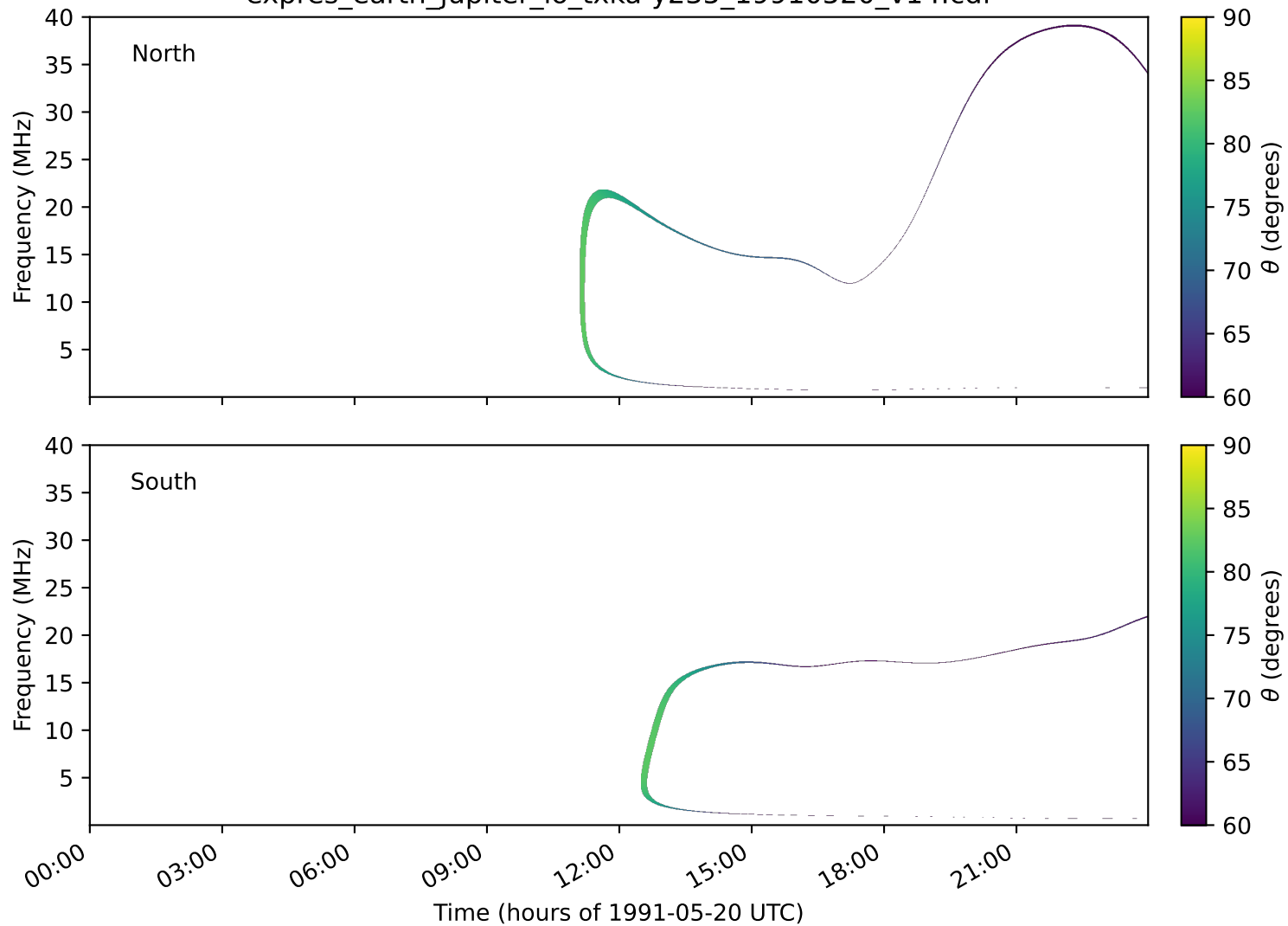
expres_earth_jupiter_io_txka-y235_19910520_v14.cdf
