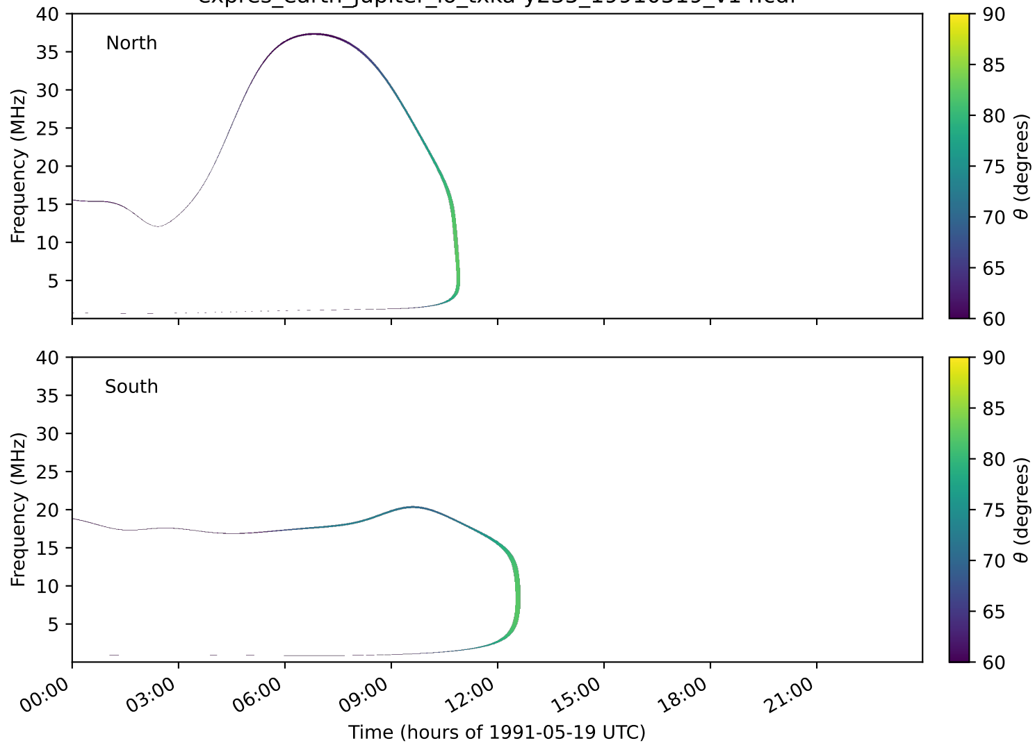
expres_earth_jupiter_io_txka-y235_19910519_v14.cdf
