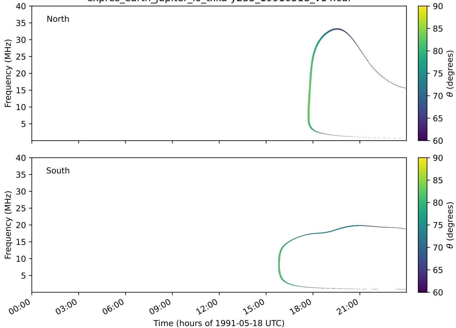
expres_earth_jupiter_io_txka-y235_19910518_v14.cdf
