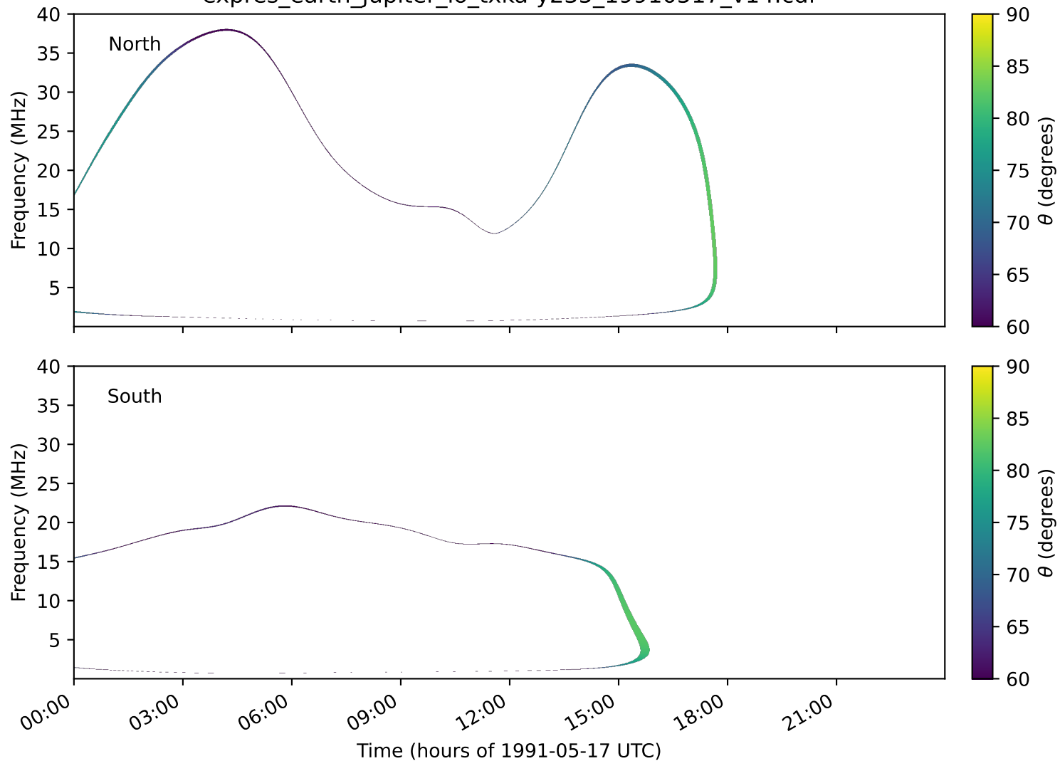
expres_earth_jupiter_io_txka-y235_19910517_v14.cdf
