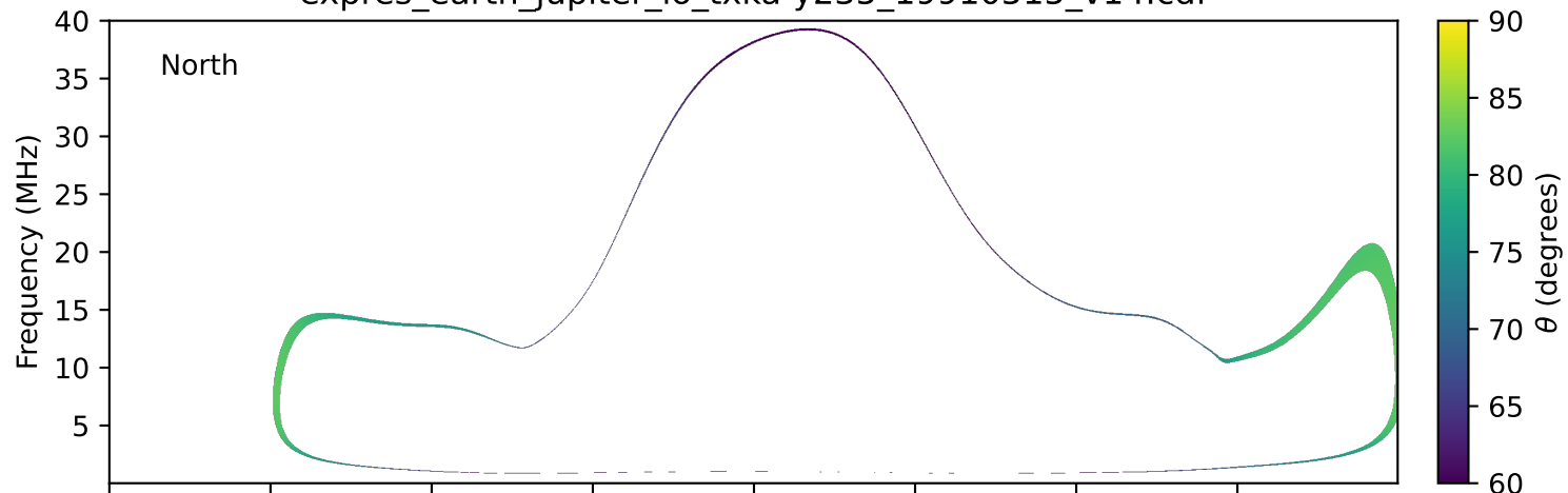
expres_earth_jupiter_io_txka-y235_19910515_v14.cdf
