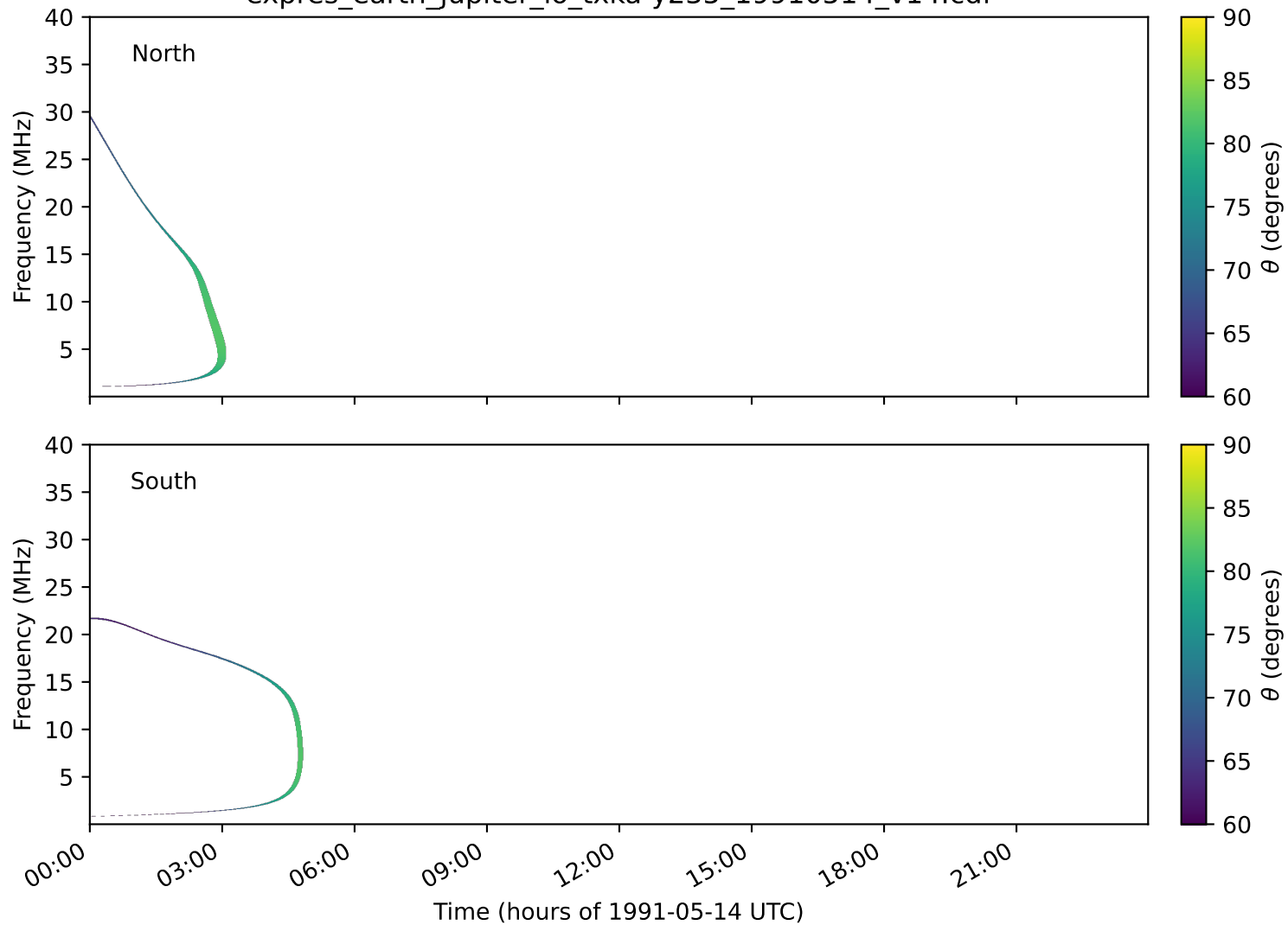
expres_earth_jupiter_io_txka-y235_19910514_v14.cdf
