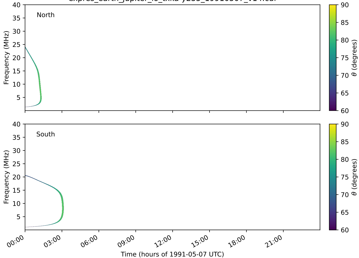
expres_earth_jupiter_io_txka-y235_19910507_v14.cdf
