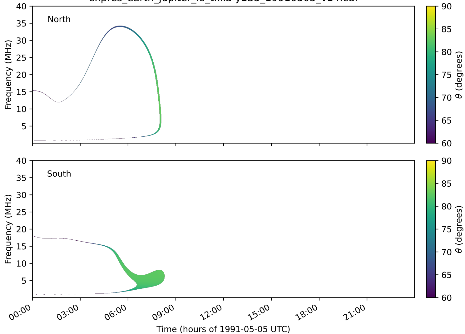
expres_earth_jupiter_io_txka-y235_19910505_v14.cdf
