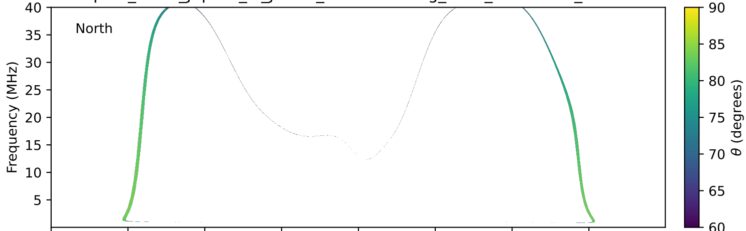
expres_earth_jupiter_io_jrm33_lossc-wid1deg_3kev_19910531_v11.cdf
