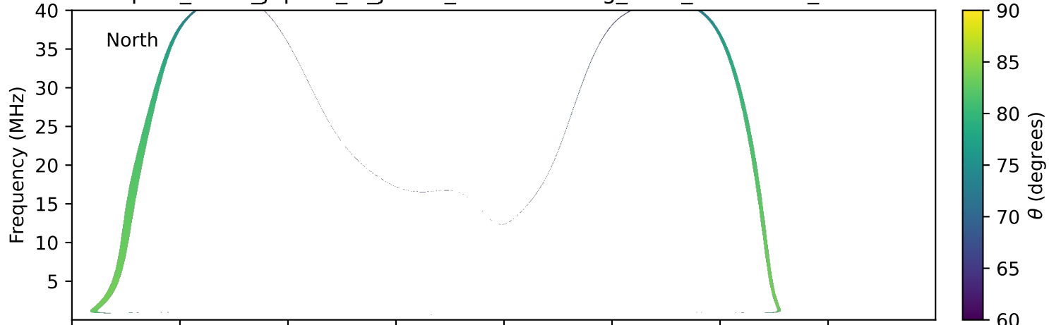
expres_earth_jupiter_io_jrm33_lossc-wid1deg_3kev_19910524_v11.cdf
