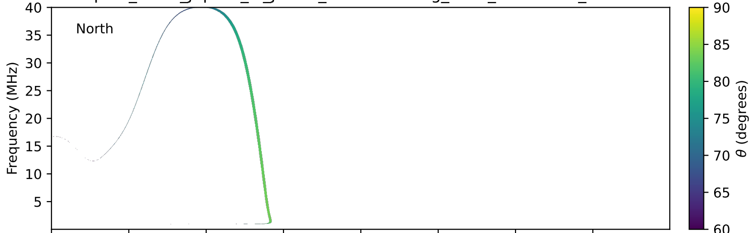
expres_earth_jupiter_io_jrm33_lossc-wid1deg_3kev_19910505_v11.cdf
