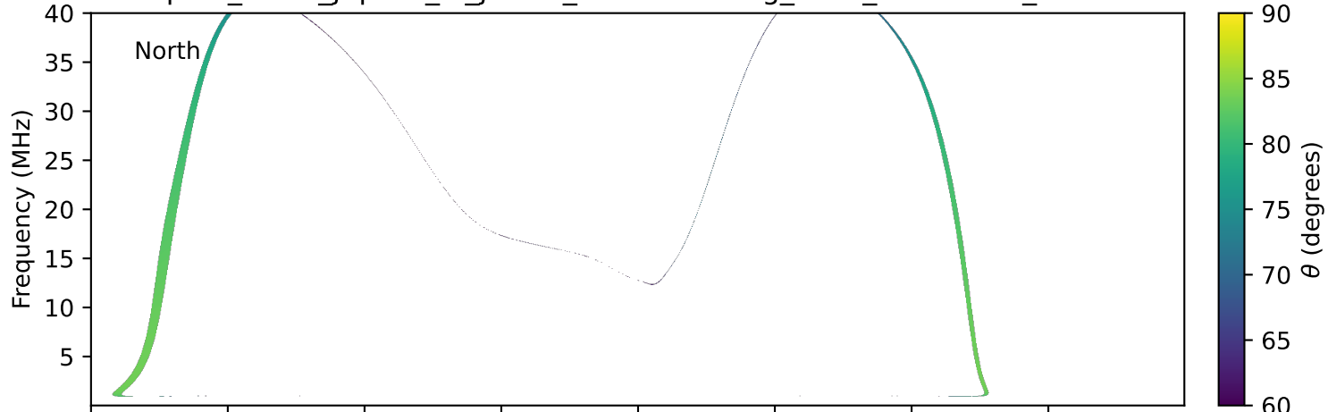
expres_earth_jupiter_io_jrm09_lossc-wid1deg_3kev_19910524_v11.cdf
