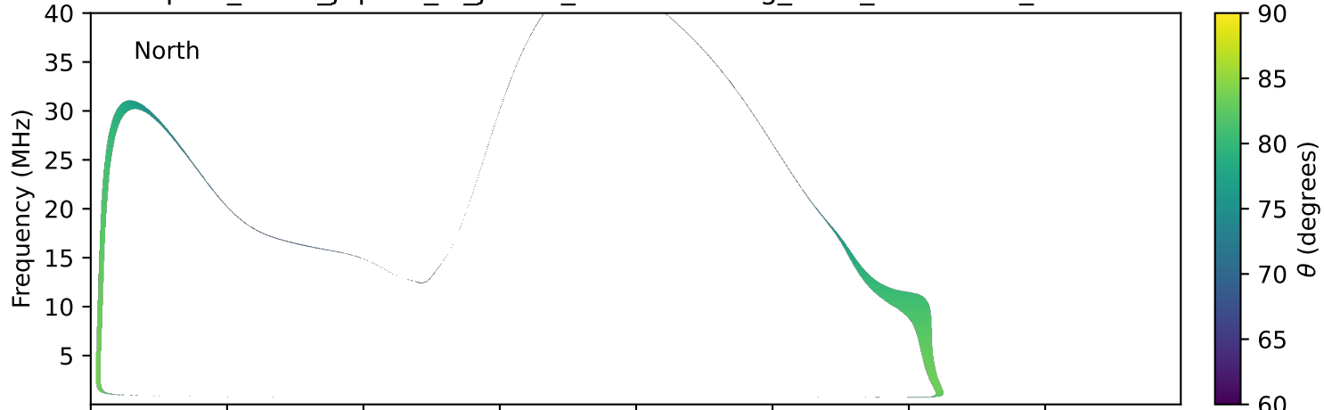
expres_earth_jupiter_io_jrm09_lossc-wid1deg_3kev_19910501_v11.cdf
