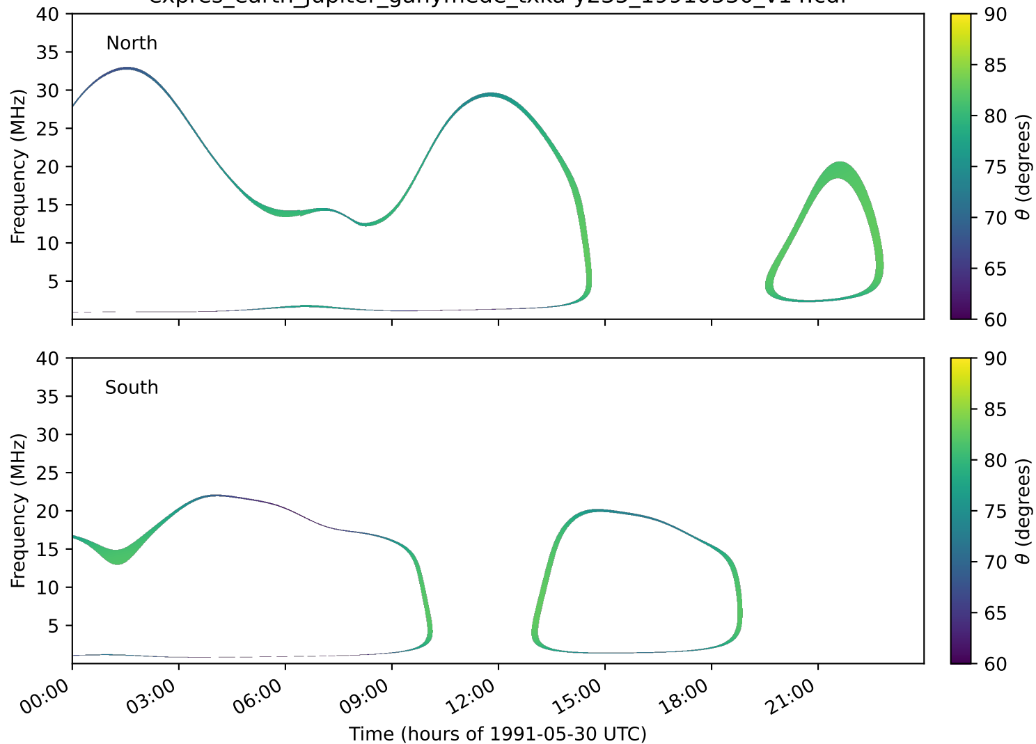
expres_earth_jupiter_ganymede_txka-y235_19910530_v14.cdf
