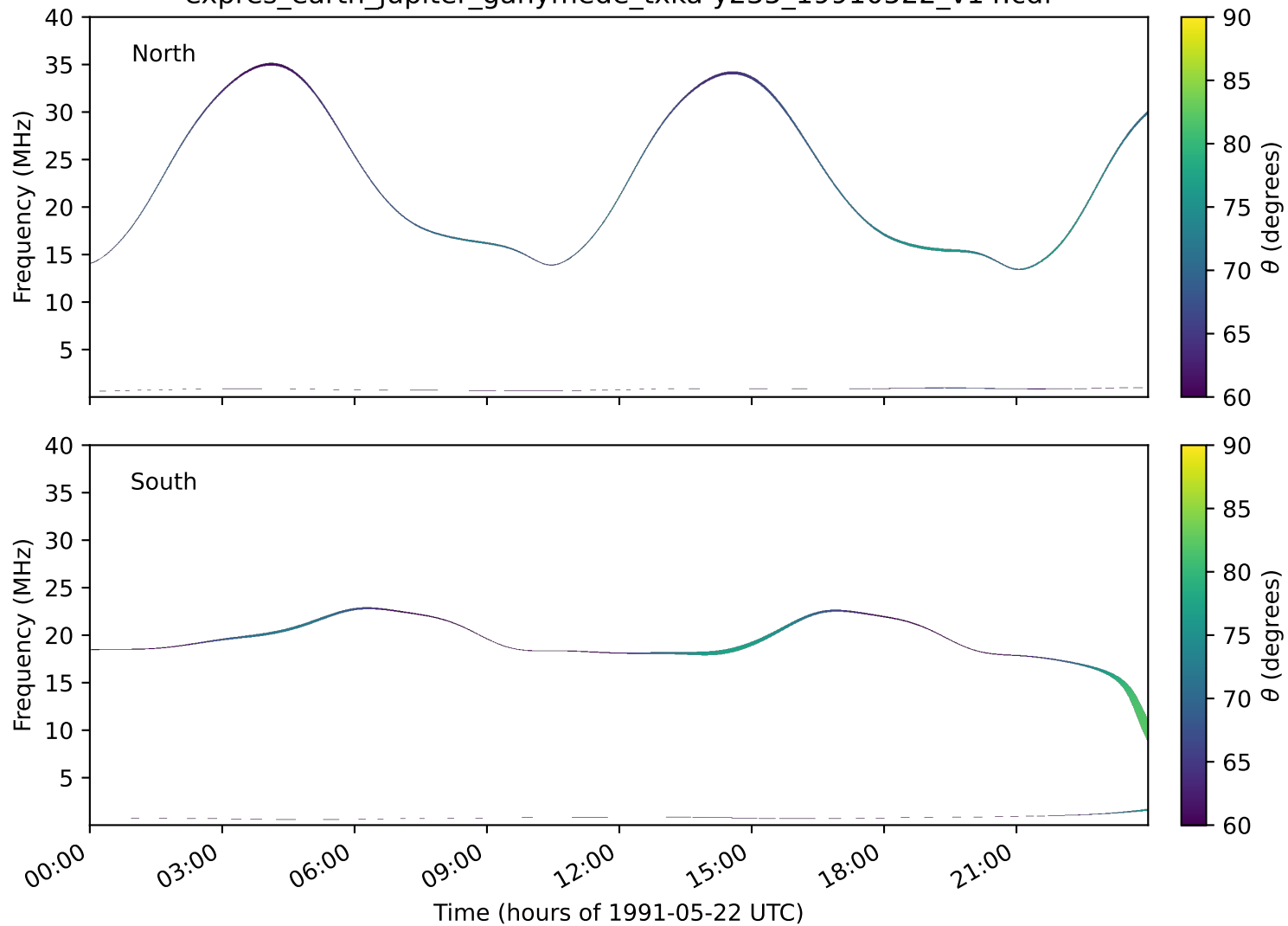
expres_earth_jupiter_ganymede_txka-y235_19910522_v14.cdf
