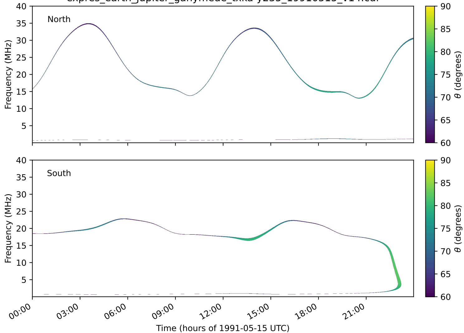
expres_earth_jupiter_ganymede_txka-y235_19910515_v14.cdf
