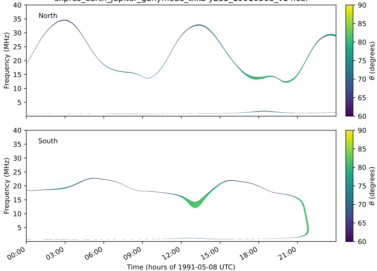
expres_earth_jupiter_ganymede_txka-y235_19910508_v14.cdf
