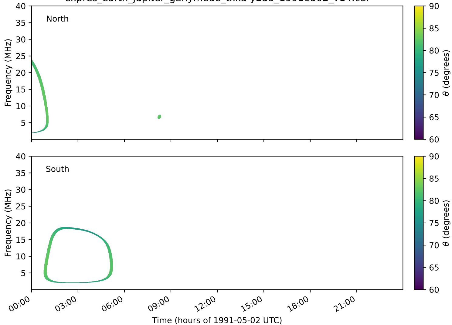
expres_earth_jupiter_ganymede_txka-y235_19910502_v14.cdf
