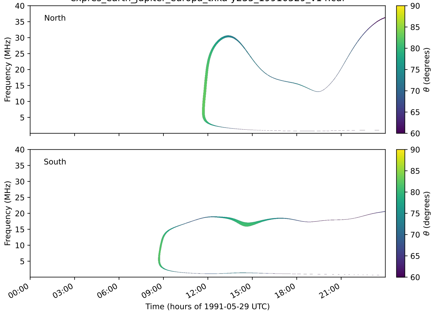
expres_earth_jupiter_europa_txka-y235_19910529_v14.cdf
