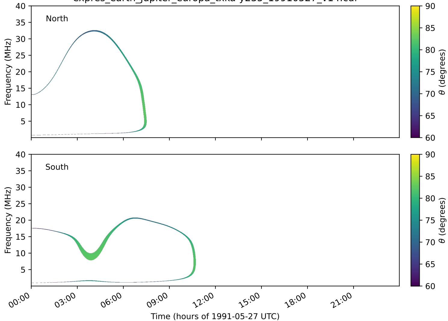
expres_earth_jupiter_europa_txka-y235_19910527_v14.cdf
