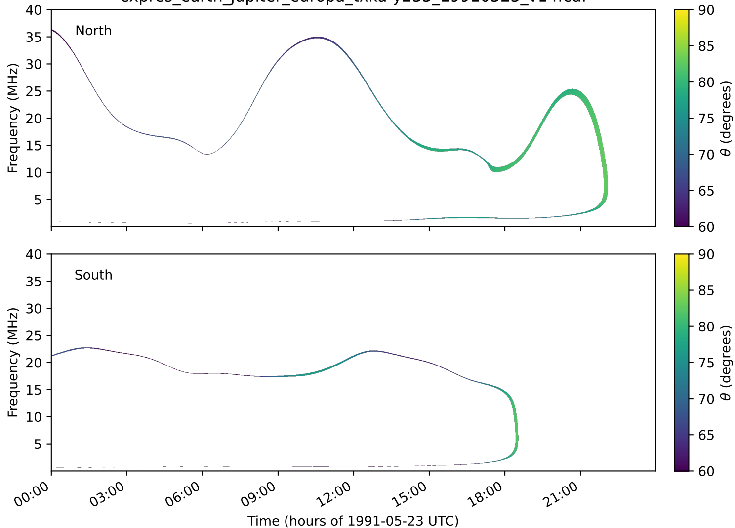
expres_earth_jupiter_europa_txka-y235_19910523_v14.cdf
