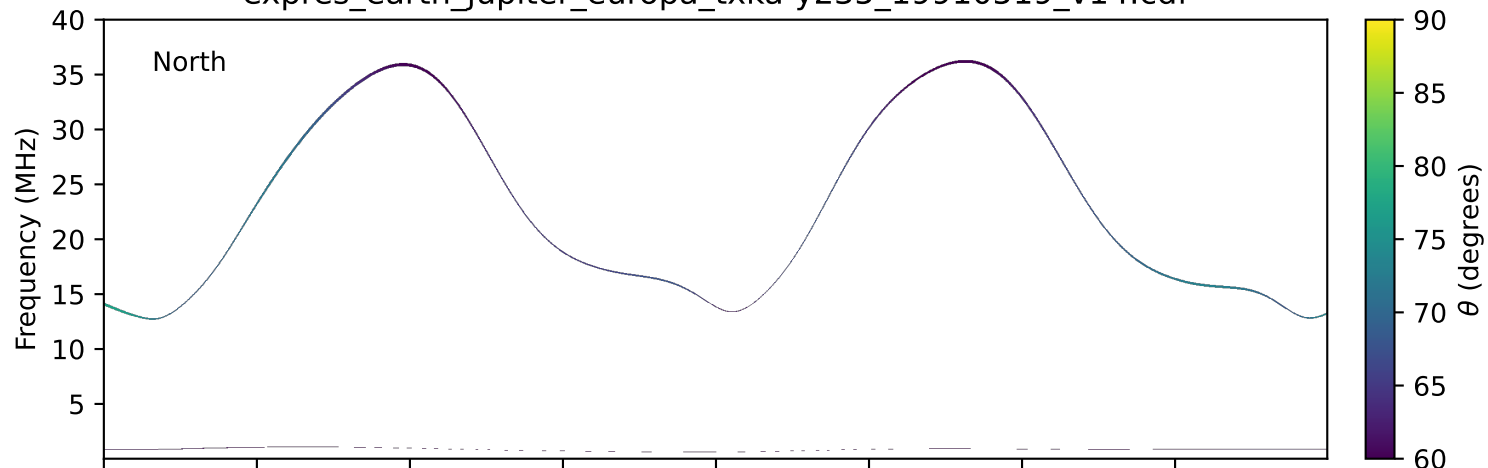
expres_earth_jupiter_europa_txka-y235_19910519_v14.cdf
