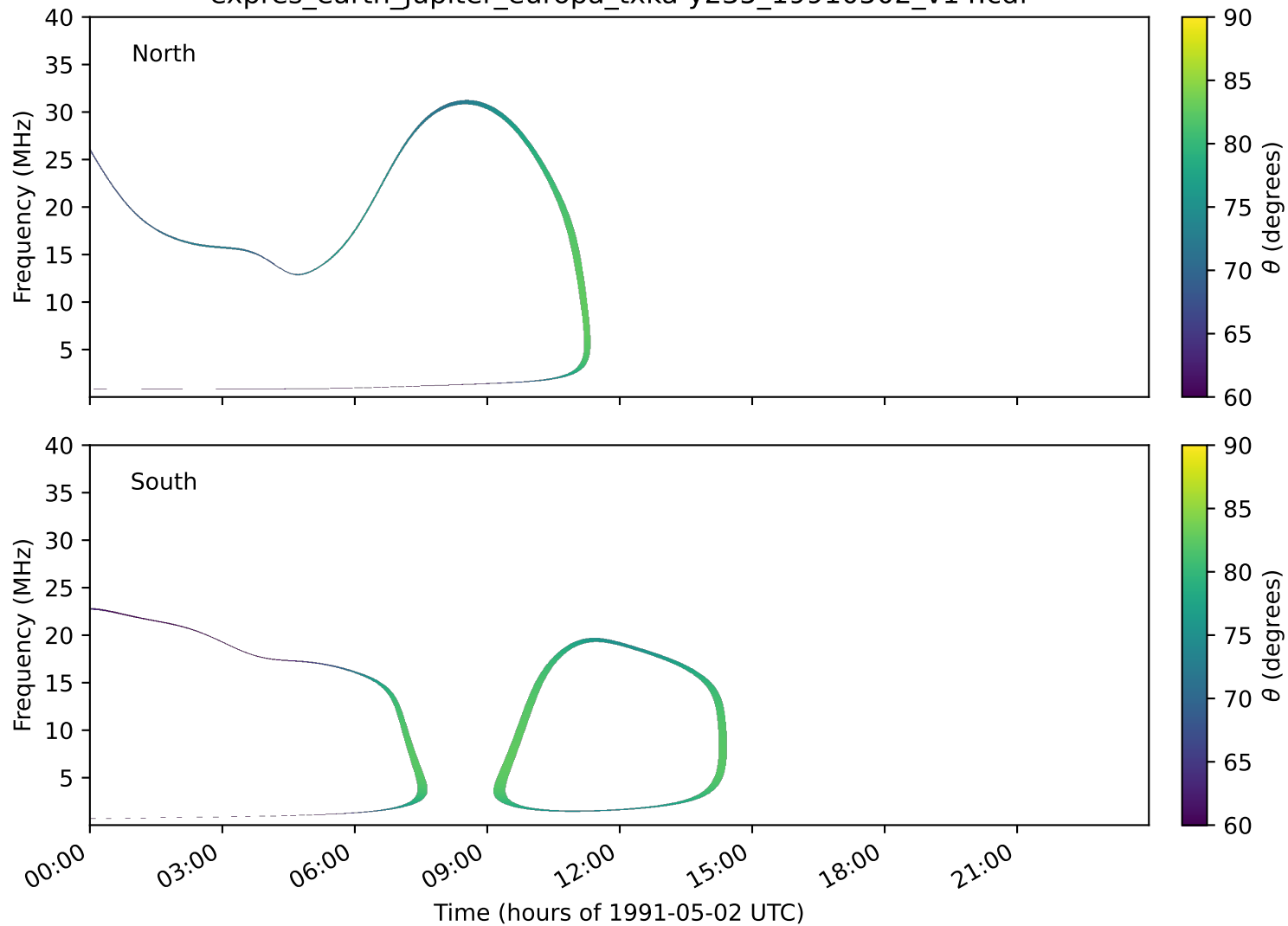
expres_earth_jupiter_europa_txka-y235_19910502_v14.cdf
