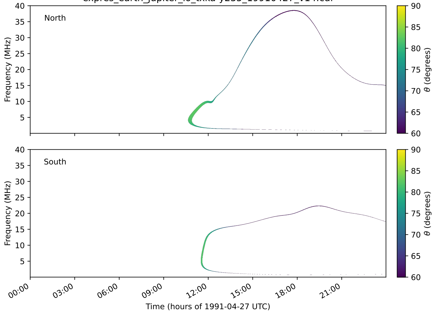
expres_earth_jupiter_io_txka-y235_19910427_v14.cdf
