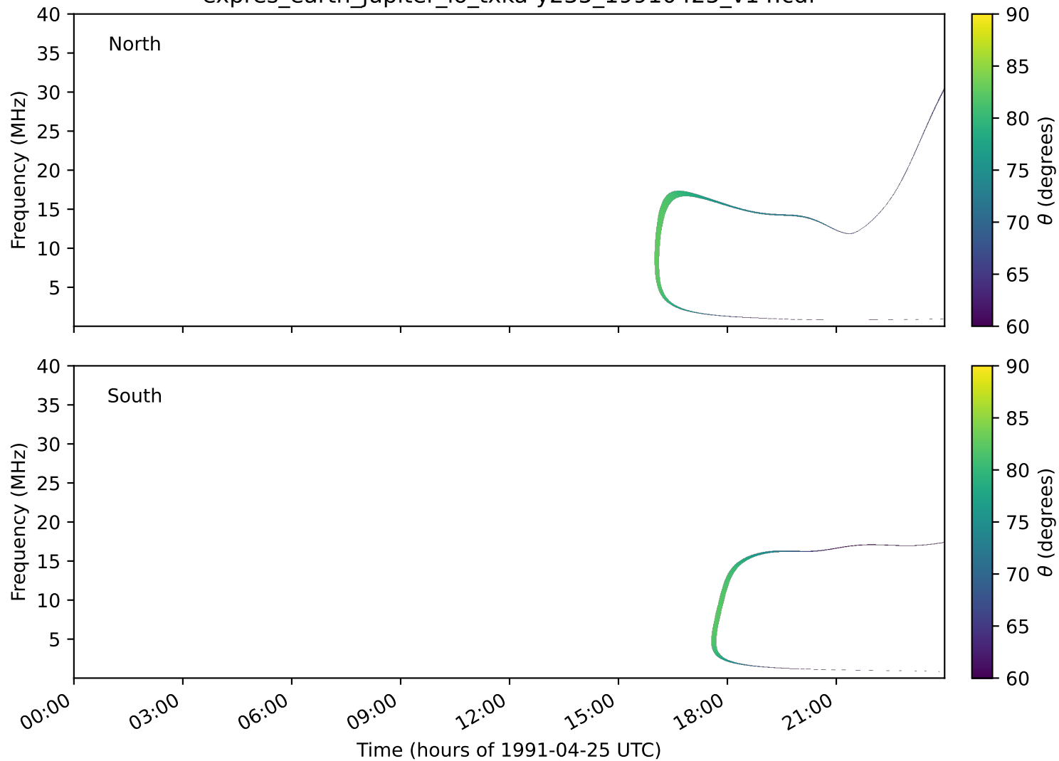
expres_earth_jupiter_io_txka-y235_19910425_v14.cdf
