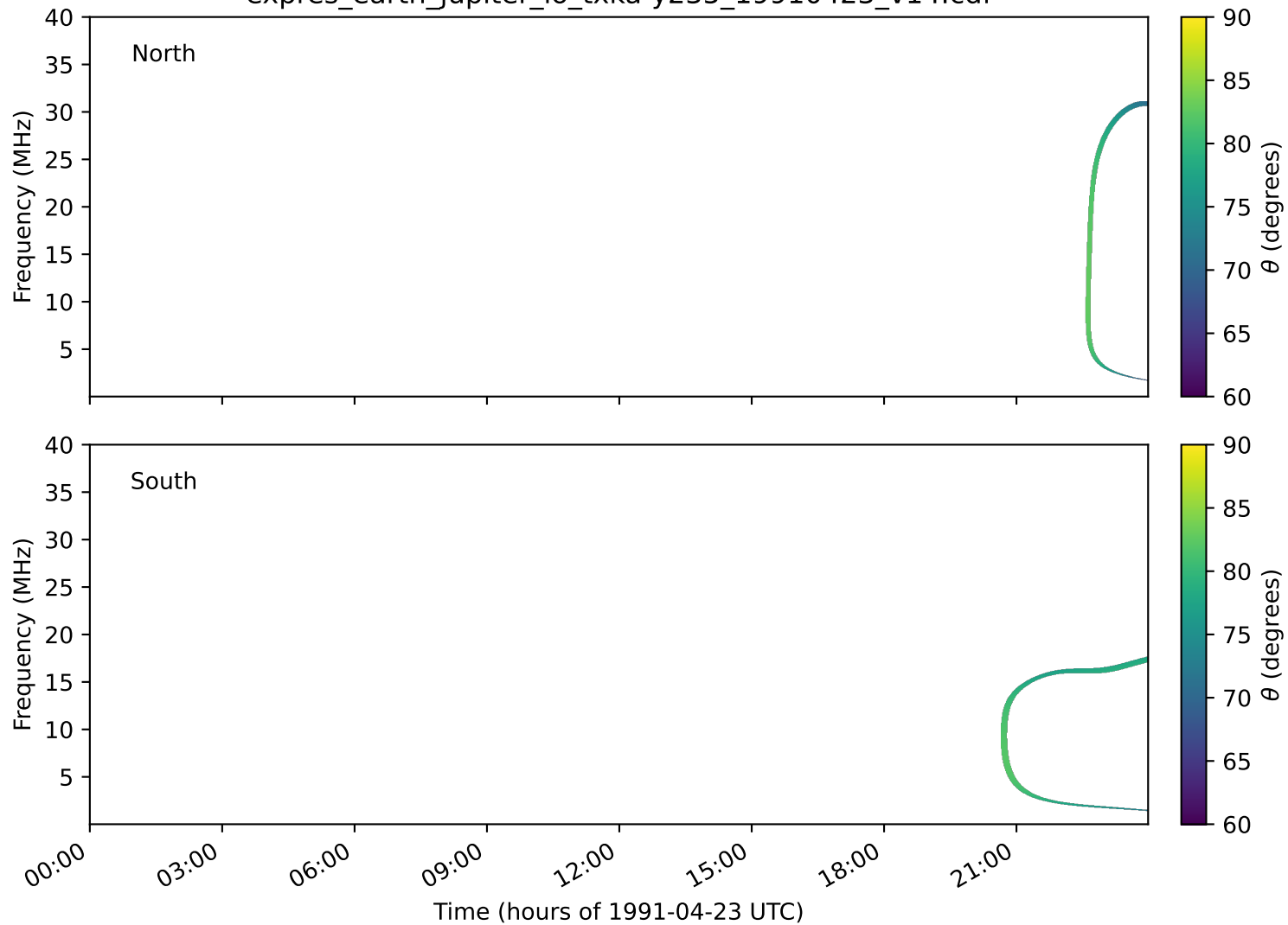
expres_earth_jupiter_io_txka-y235_19910423_v14.cdf
