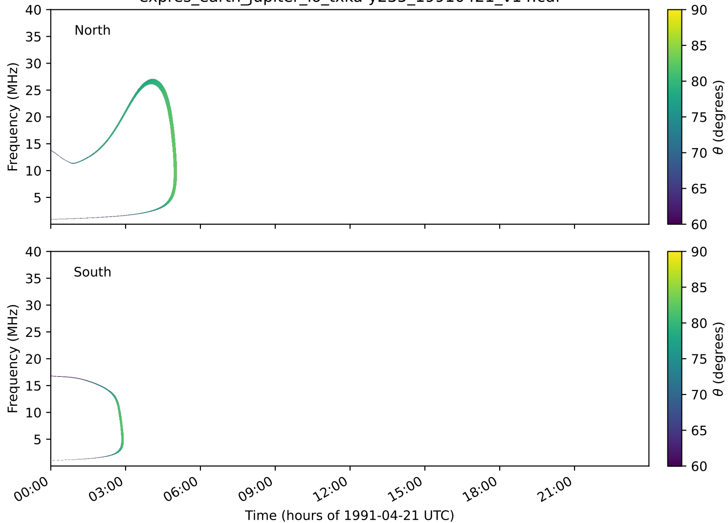
expres_earth_jupiter_io_txka-y235_19910421_v14.cdf
