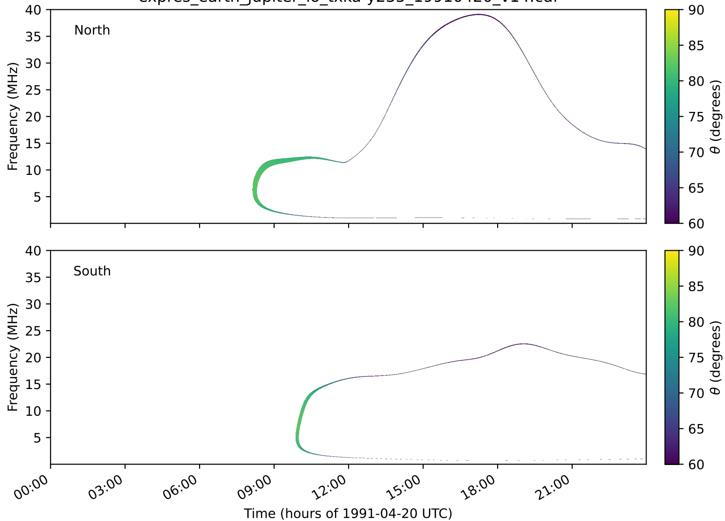
expres_earth_jupiter_io_txka-y235_19910420_v14.cdf
