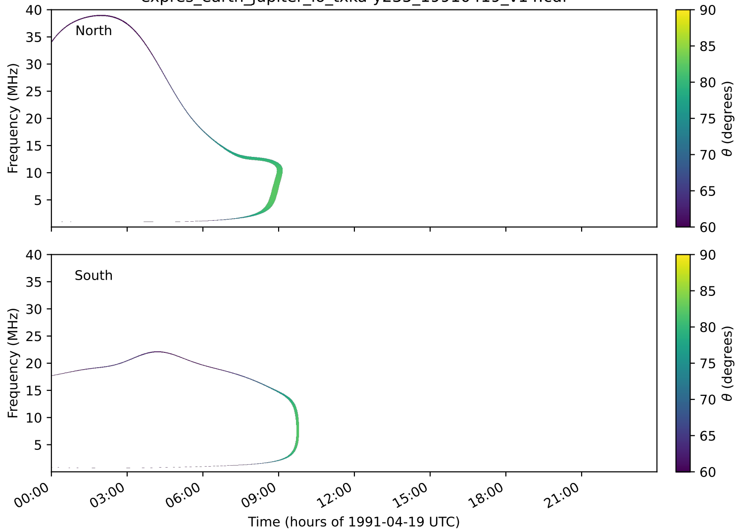
expres_earth_jupiter_io_txka-y235_19910419_v14.cdf
