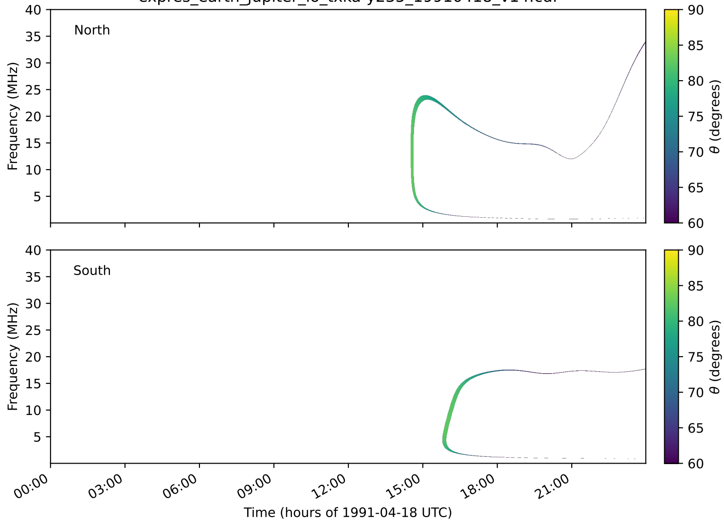
expres_earth_jupiter_io_txka-y235_19910418_v14.cdf
