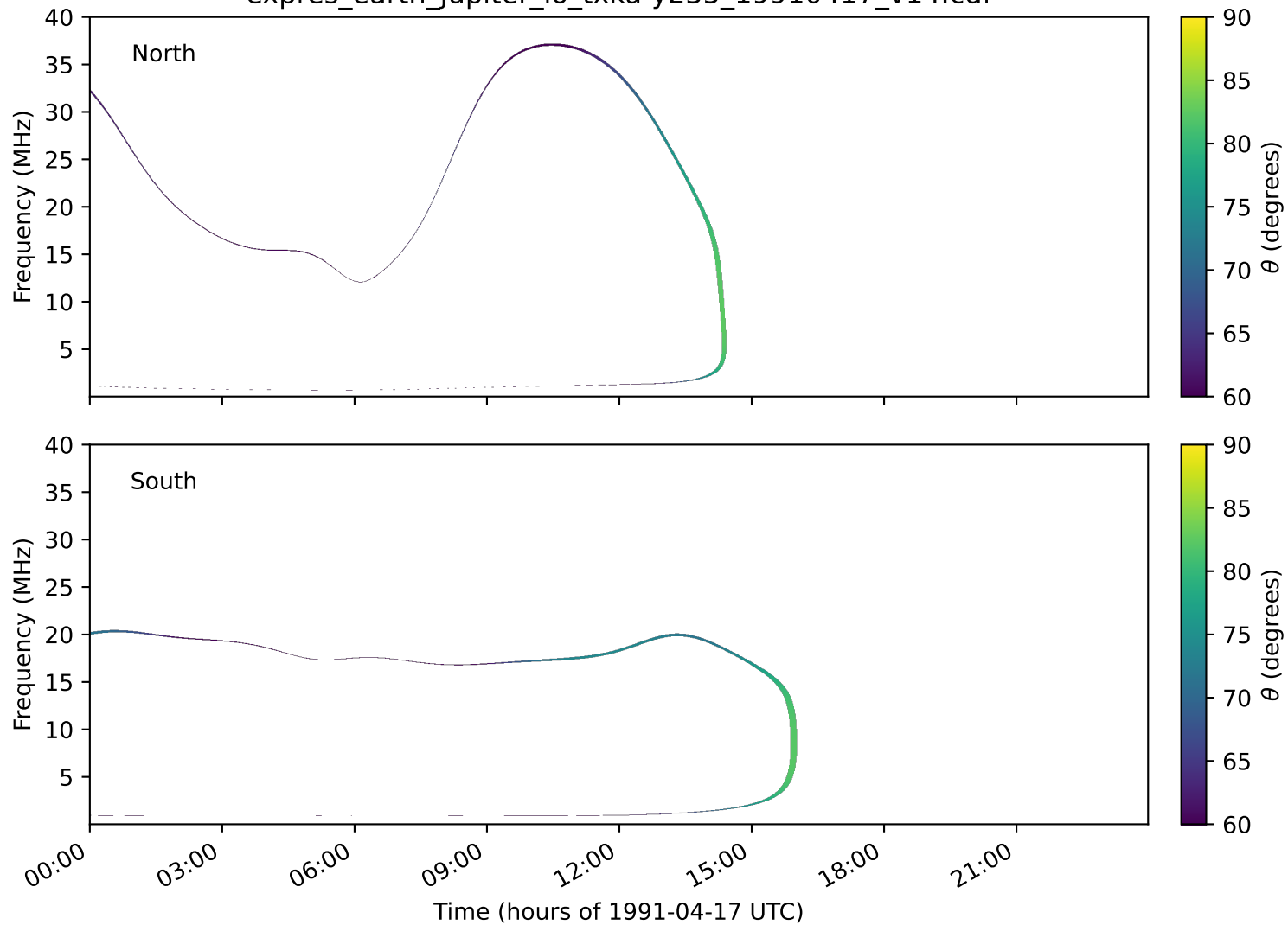
expres_earth_jupiter_io_txka-y235_19910417_v14.cdf
