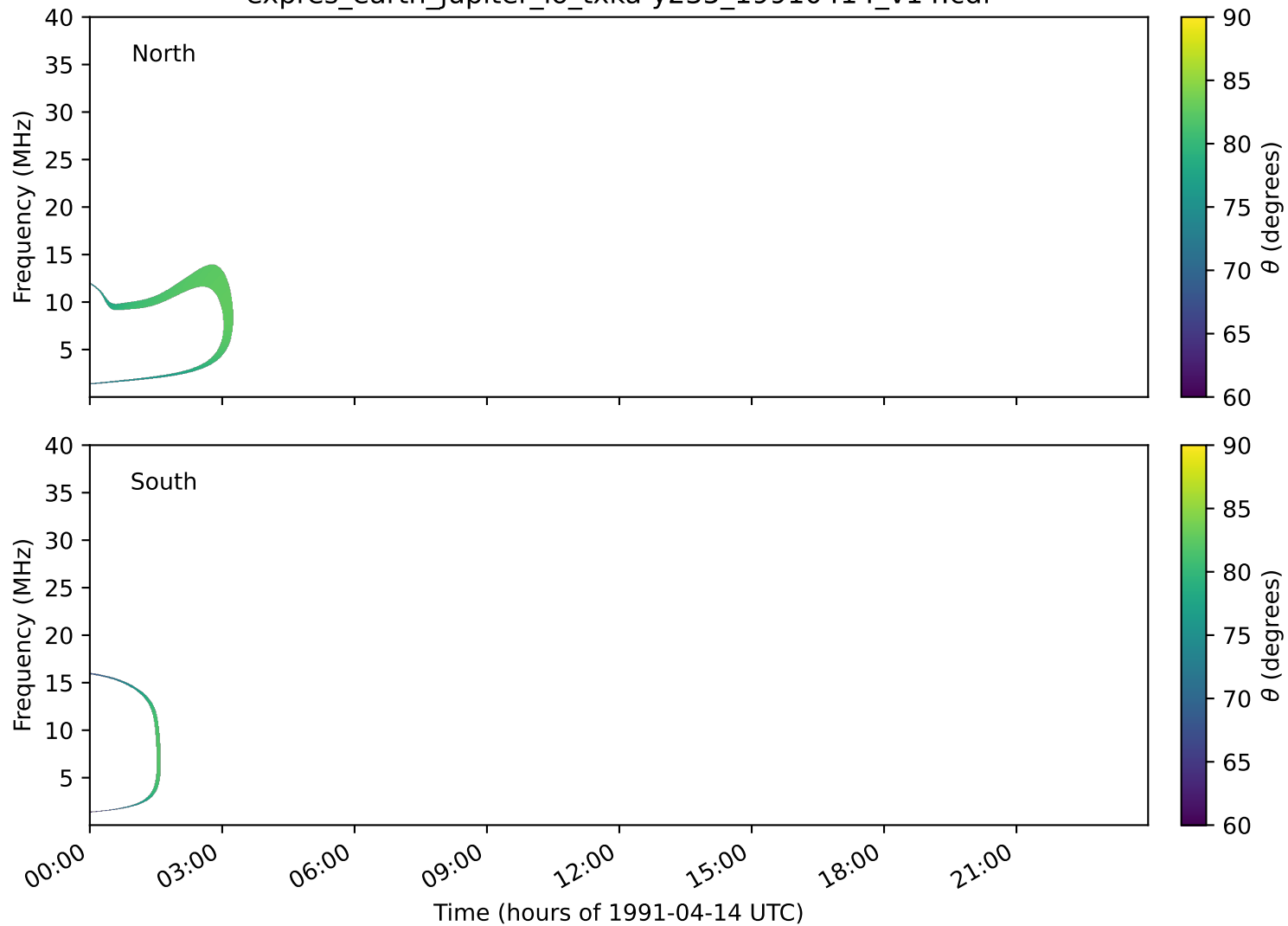
expres_earth_jupiter_io_txka-y235_19910414_v14.cdf
