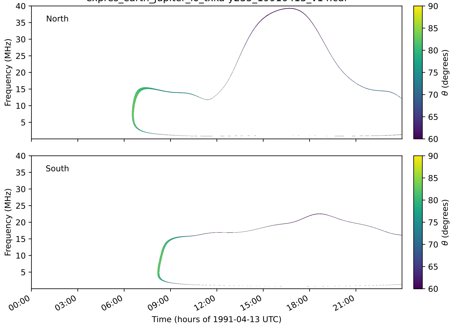
expres_earth_jupiter_io_txka-y235_19910413_v14.cdf
