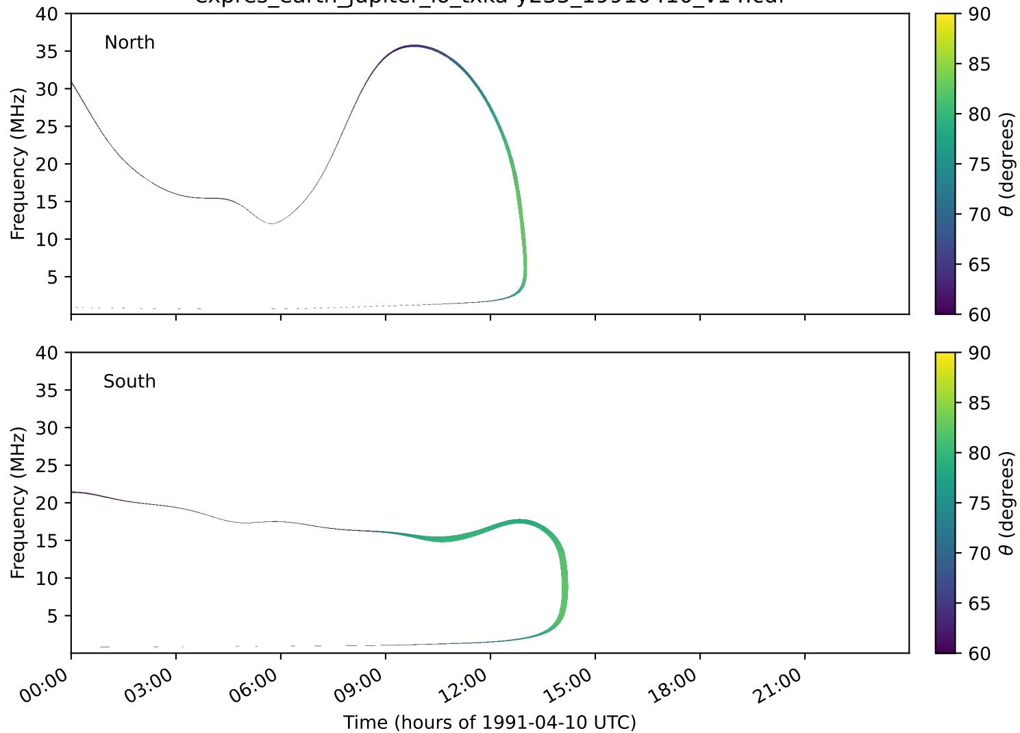
expres_earth_jupiter_io_txka-y235_19910410_v14.cdf
