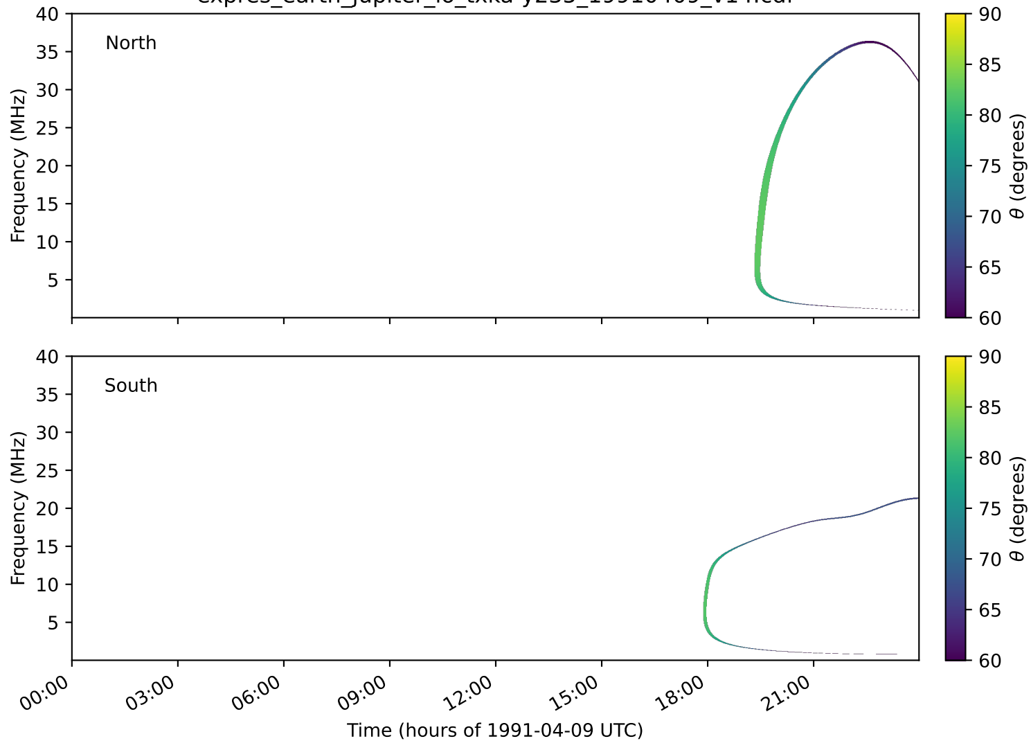
expres_earth_jupiter_io_txka-y235_19910409_v14.cdf
