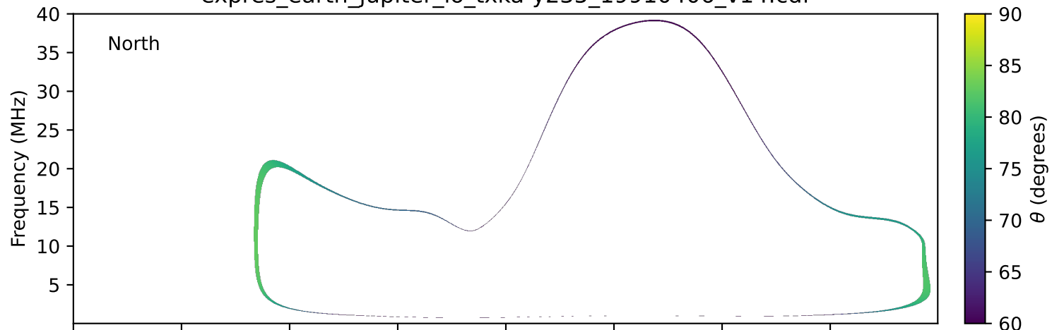
expres_earth_jupiter_io_txka-y235_19910406_v14.cdf
