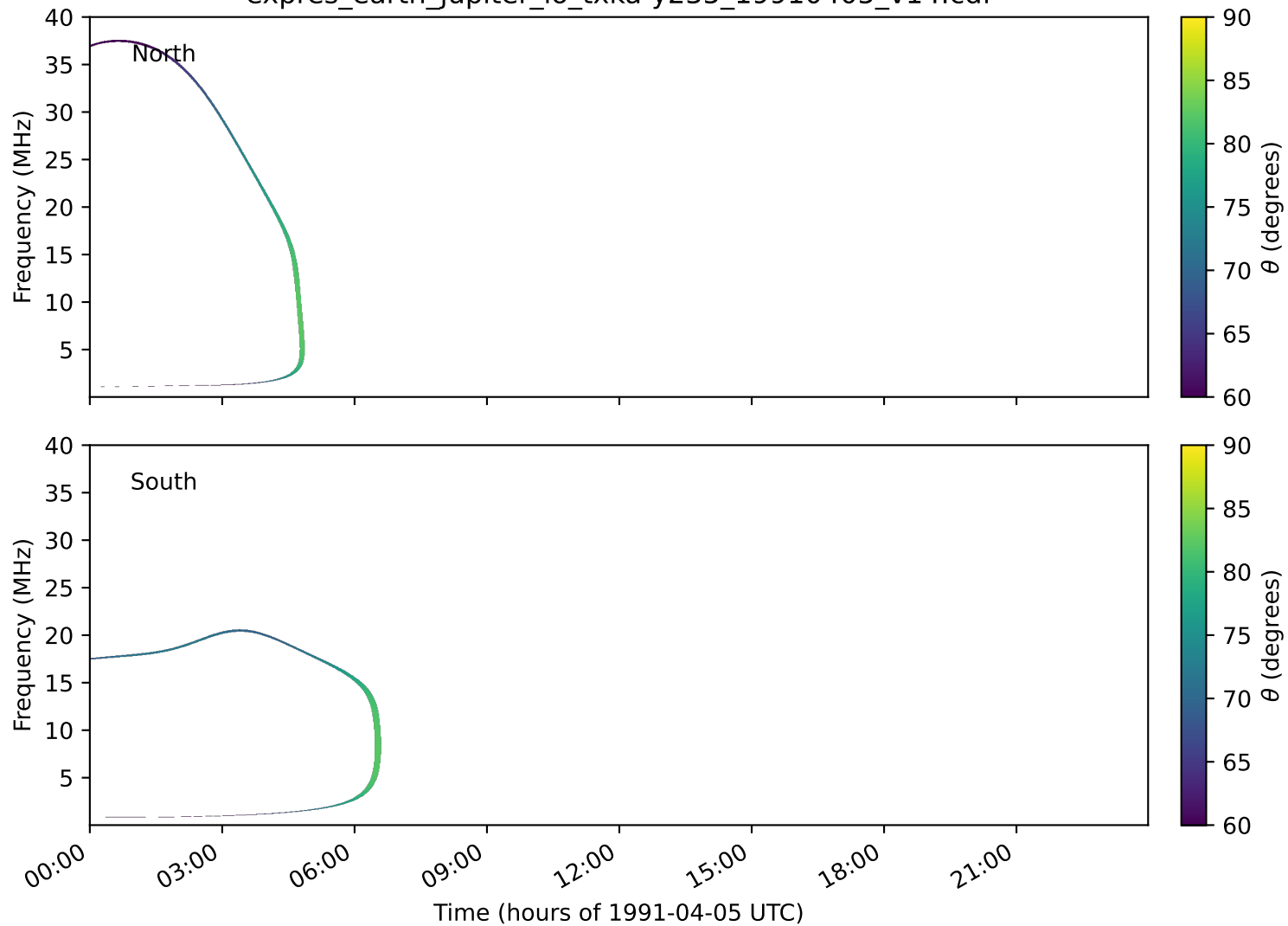
expres_earth_jupiter_io_txka-y235_19910405_v14.cdf
